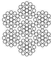
FIGURE 52. Type VI, small cord, class 3, 7 by 19 (2 operations).
