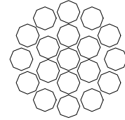
FIGURE 49. Type V, auxillary wire strands, class 2, 1 by 19 seizing strand (2 operations).
